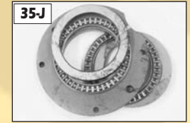
Thrust Bearing Axial Kit #00.550.0433
