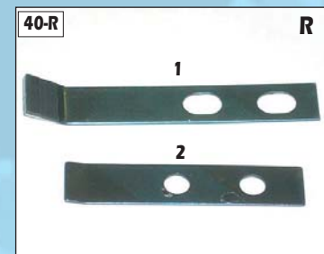
1. Delivery Carriage Gripper Finger #S 1415F 2. Backing Plate #S 1411F
