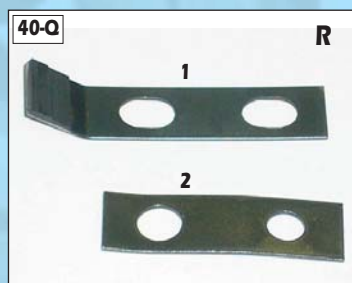
1. Delivery Gripper Finger #S 1404F 2. Backing Plate #S 1441
