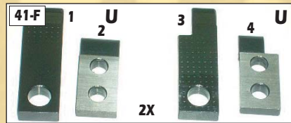
41-F 1 U 2 U 3 U 4 U 1. Pincer/Perfect/fixed/lower #52.580.338 2. Pincer/Perfect/moveable/top-M #52.580.337 3. Pincer/Perfect/fixed/lower/cut out #52.580.363 4. Pincer/Perfect/moveable/top/cut out #52.580.362
