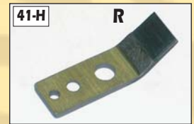
41-H R Delivery Gripper Finger #14.875.001 Backing Plate #14.014.041
