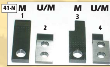
41-N 1 M 2 U/M 3 M 4 U/M 1. Pincer/Perfect/fixed/lower-M #52.580.338 2a. Pincer/Perfect/moveable/ top-M #52.580.337 2b. Pincer/Perfect/moveable/top U #79.580.337 3. Pincer/Perfect/fixed/lower/cut-out-M #52.580.363 4a. Pincer/Perfect/moveable/top/cut-out-M #52.580.362 4b. Pincer/Perfect/moveable/top/cut-out-U #79.580.662
