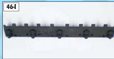
46-I Impression Cylinder Gripper Pad – Straight Cut GTO52 #69.011.008 GTO46 #42.011.008
