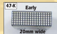
47-K Early 20mm wide #2 Transfer (After Double Drum – Straight Printing) #58.011.020 – straight – parallel #58.711.101 – cross grooved
