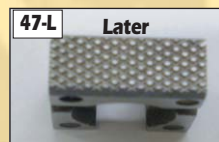
47-L Later Narrow 18mm wide x 18mm high #91.014.310
