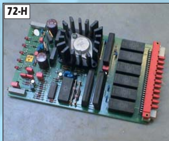
PCB Ink Key Motor #71.186.4361
