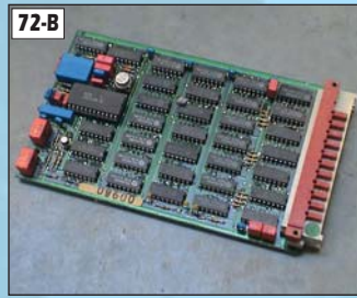
PCB For Circumferential Register 4 Zones #71.186.3341
