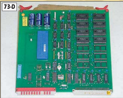
SPK #81.186.5355 Memory
