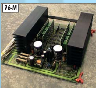
LTK-500 #91.144.8062
