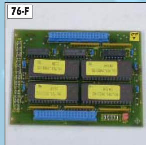
SRK EPHROM-4 #91.150.0061
