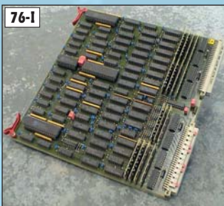
SEK #91.144.6041
