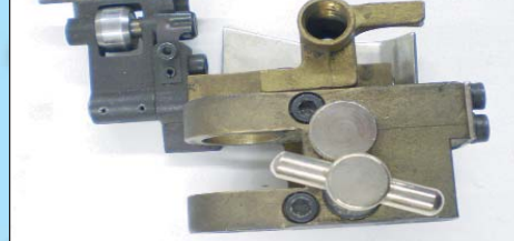
Side Guide Ass'y - Drive Side AKA Bearing D.S. #53.072.203
