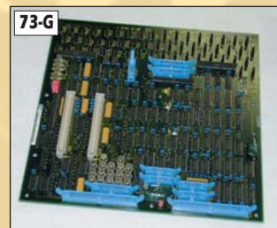
73-G ATV Display & Keyboard Distribution #81.186.5515
