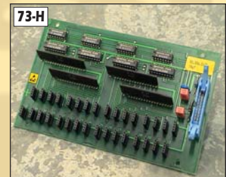
73-H FZT Distribution PCB for ink zone keys #81.186.5625
